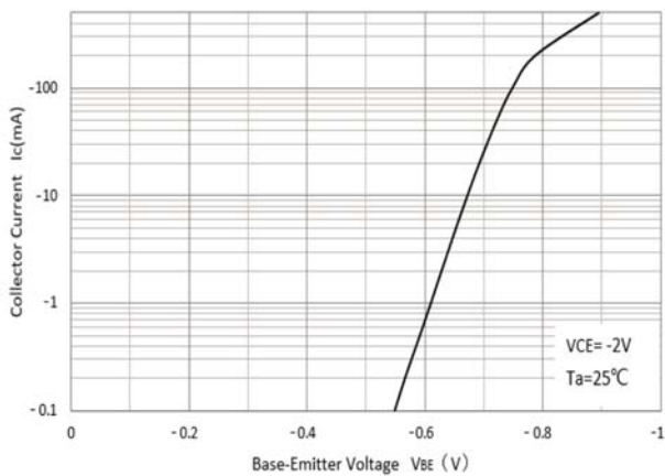
Fig 5: Base-Emittor Voltage
