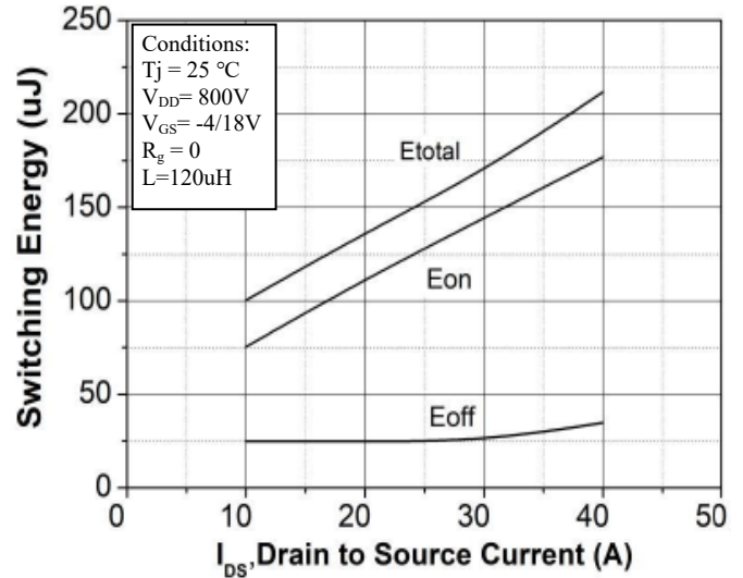
Figure 20. Clamped Inductive switching energy vs. drain current
