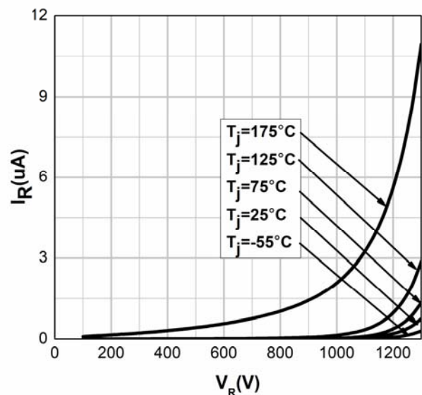
Figure 2. Reverse Characteristics
