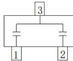
BAS70-06Q Marking:76
